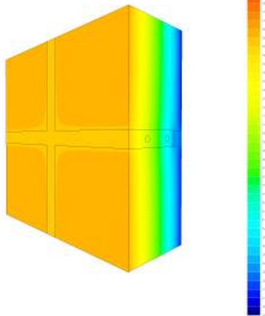
Figure 1: Isothermal lines Glass Block Wall Type 1919/8 Energy Saving Glass Block
